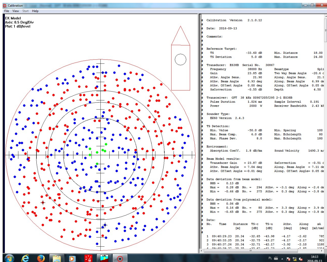
Figure 3.4.1. An example (a screenshot) of coverage of the beam area during calibration process of the Simrad EK-60 with 38 kHz transducer, performed on 13.09.2016 by the r.v. "Baltica".
